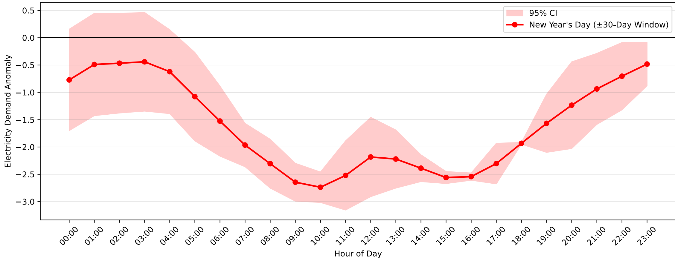
Lidcombe Demand Anomaly: New Year's Day (2016–2017, \pm 30 -Day Window)
