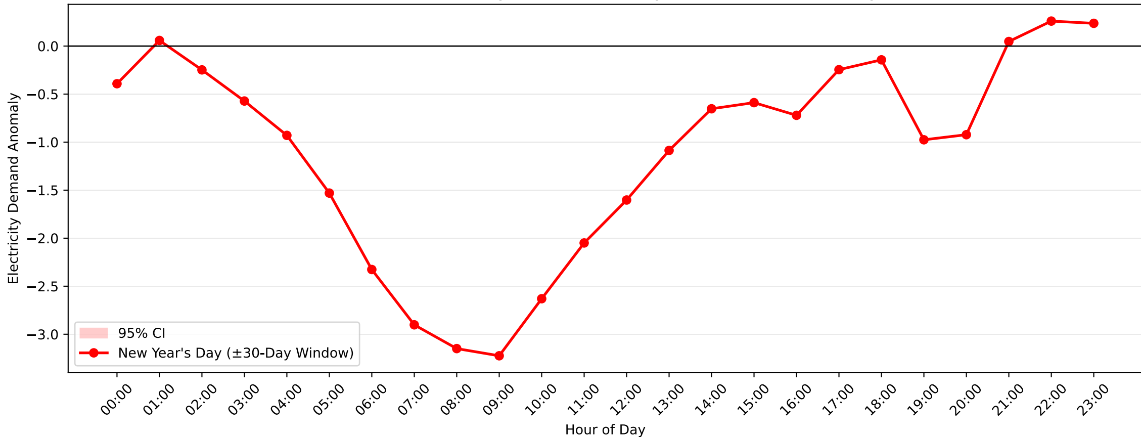
Lidcombe Demand Anomaly: New Year's Day (2010-2011, \pm 30 -Day Window)
