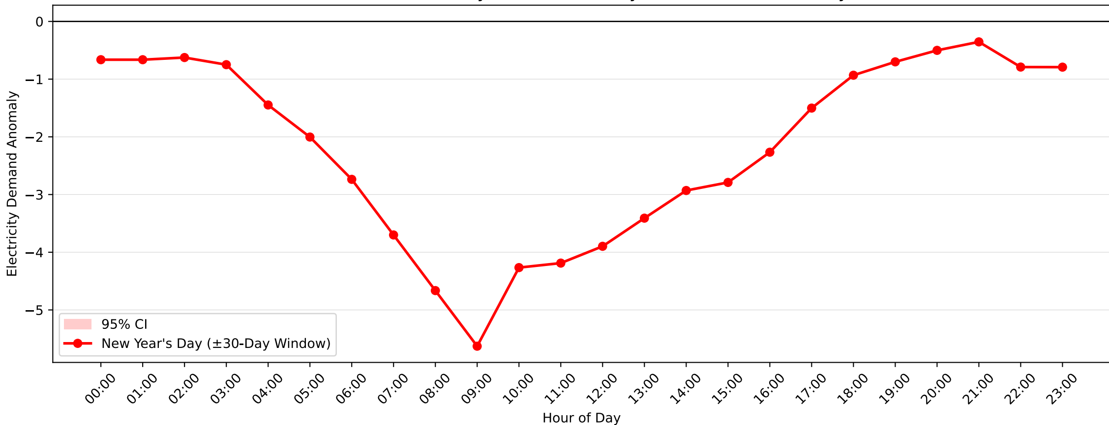
Lidcombe Demand Anomaly: New Year's Day (2009-2010, \pm 30 -Day Window)
