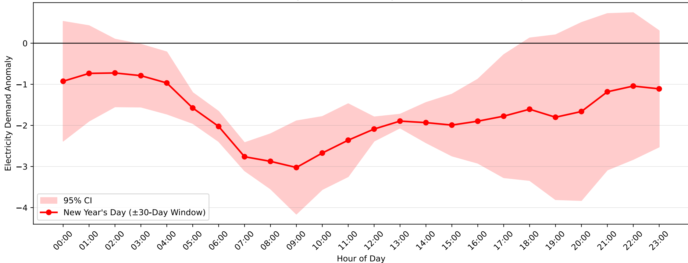
Lidcombe Demand Anomaly: New Year's Day (2012-2013, \pm 30 -Day Window)
