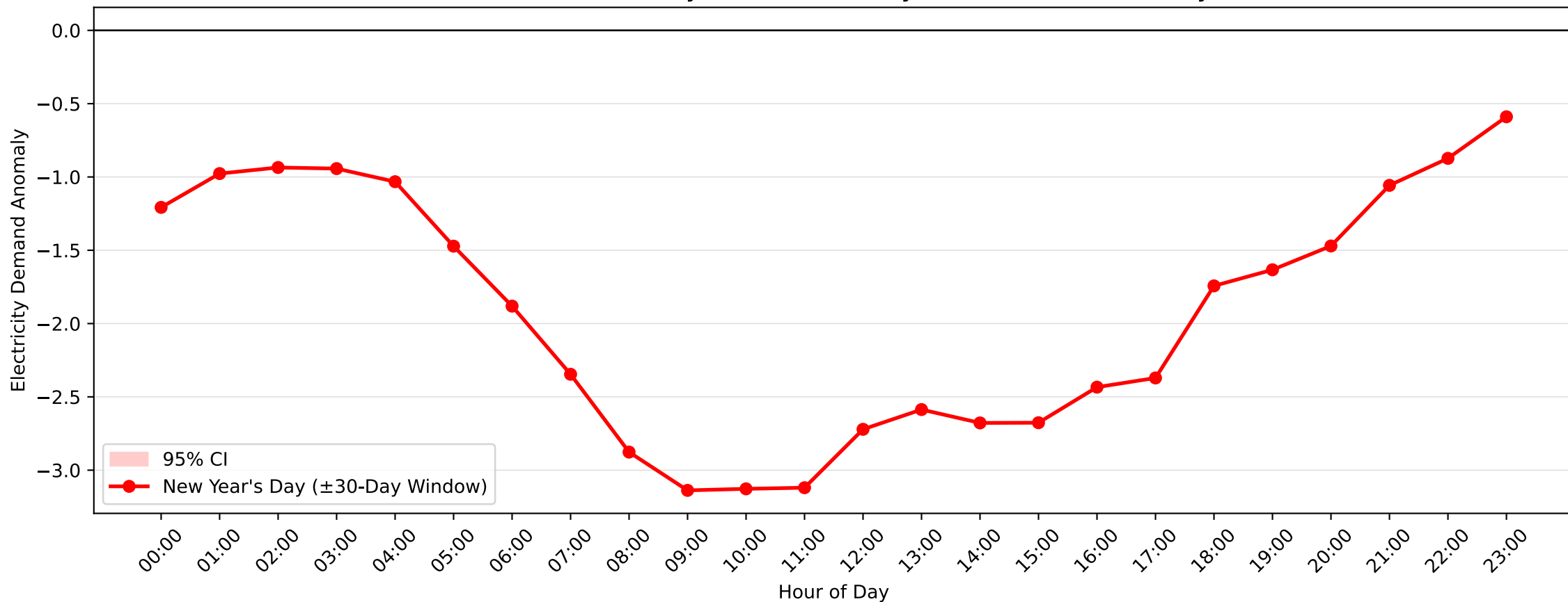
Lidcombe Demand Anomaly: New Year's Day (2015–2016, \pm 30 -Day Window)
