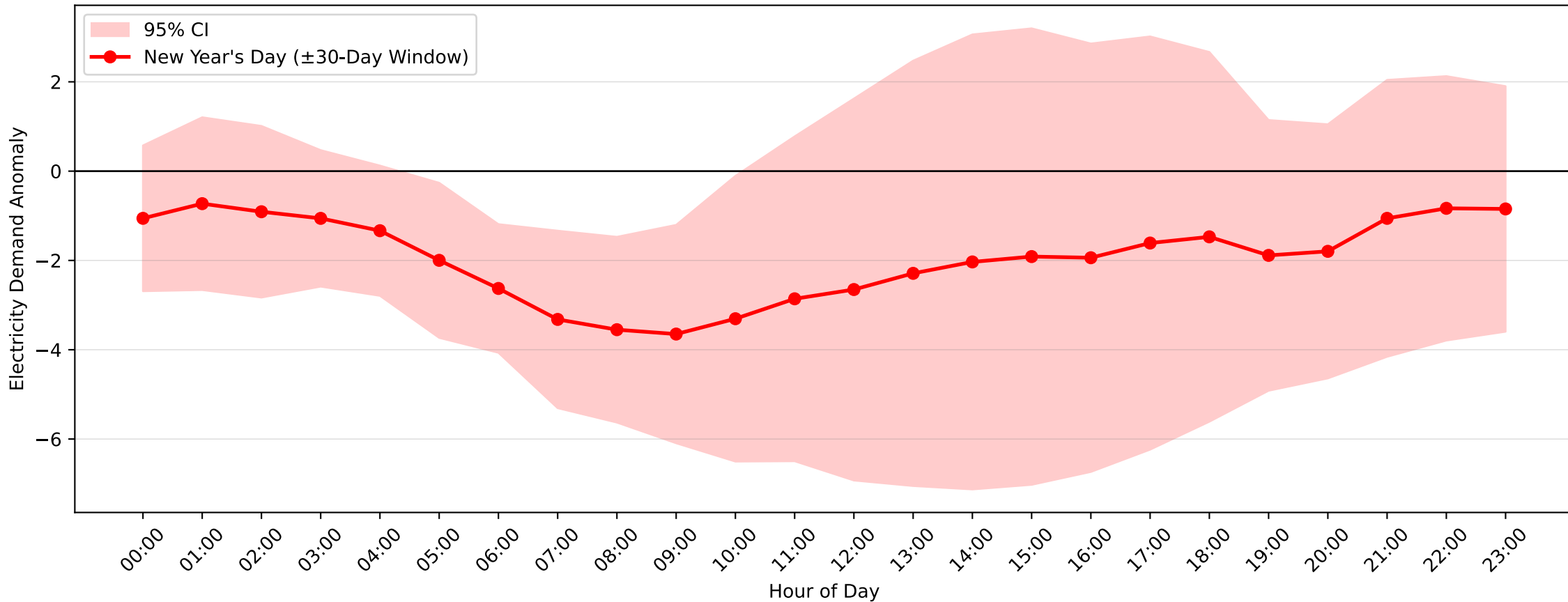
Lidcombe Demand Anomaly: New Year's Day (2011-2012, \pm 30 -Day Window)
