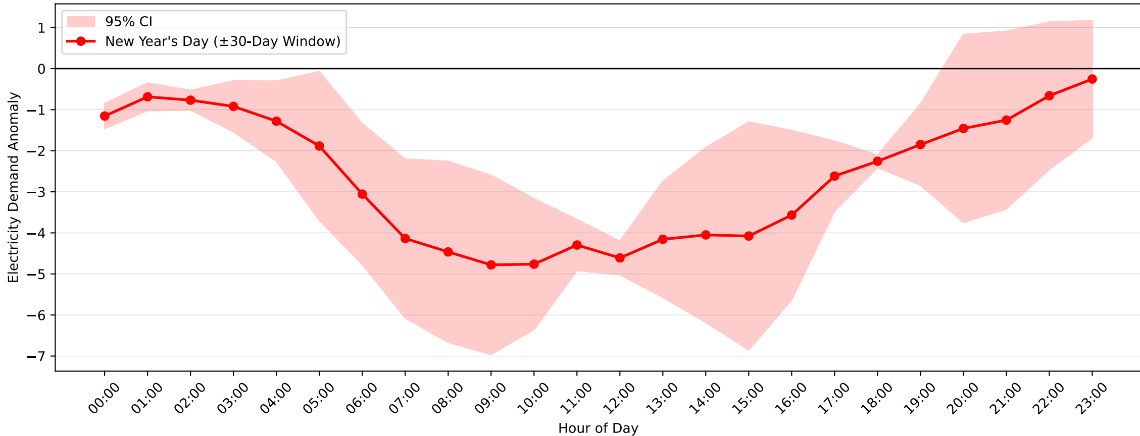
Lidcombe Demand Anomaly: New Year's Day (2004-2005, \pm 30 -Day Window)
