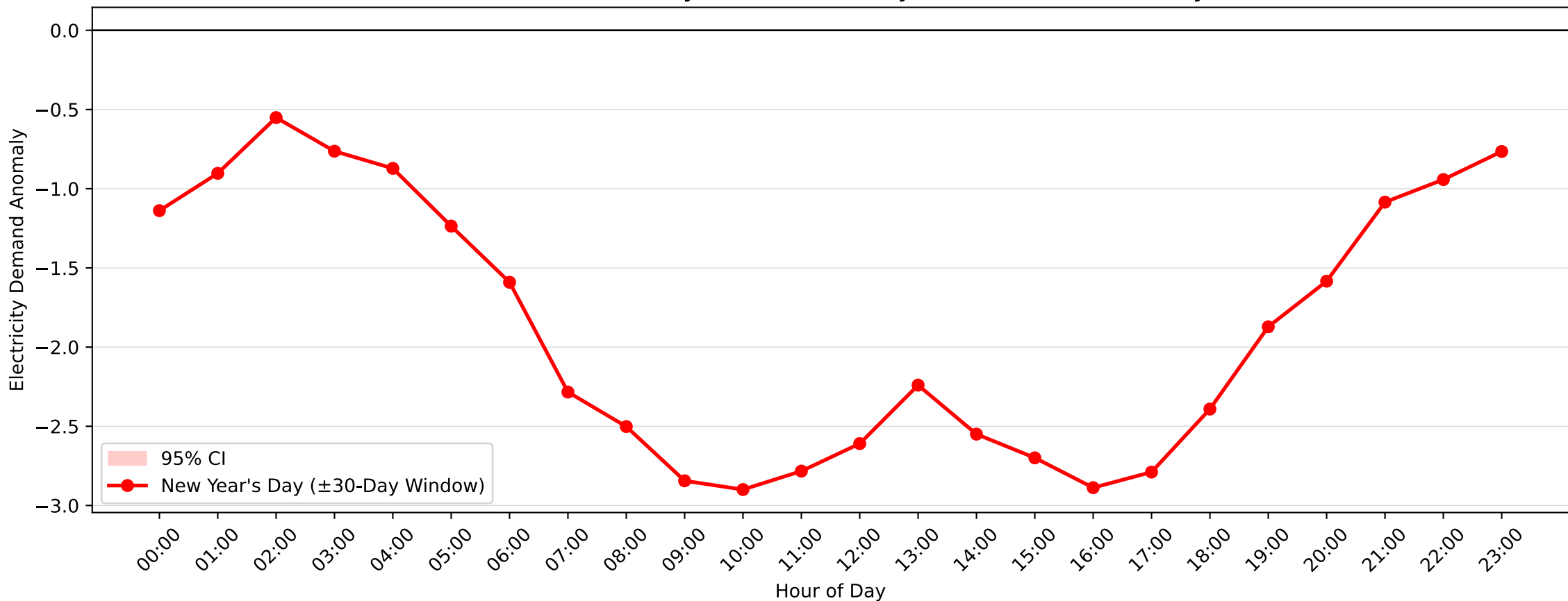
Lidcombe Demand Anomaly: New Year's Day (2014–2015, \pm 30 -Day Window)
