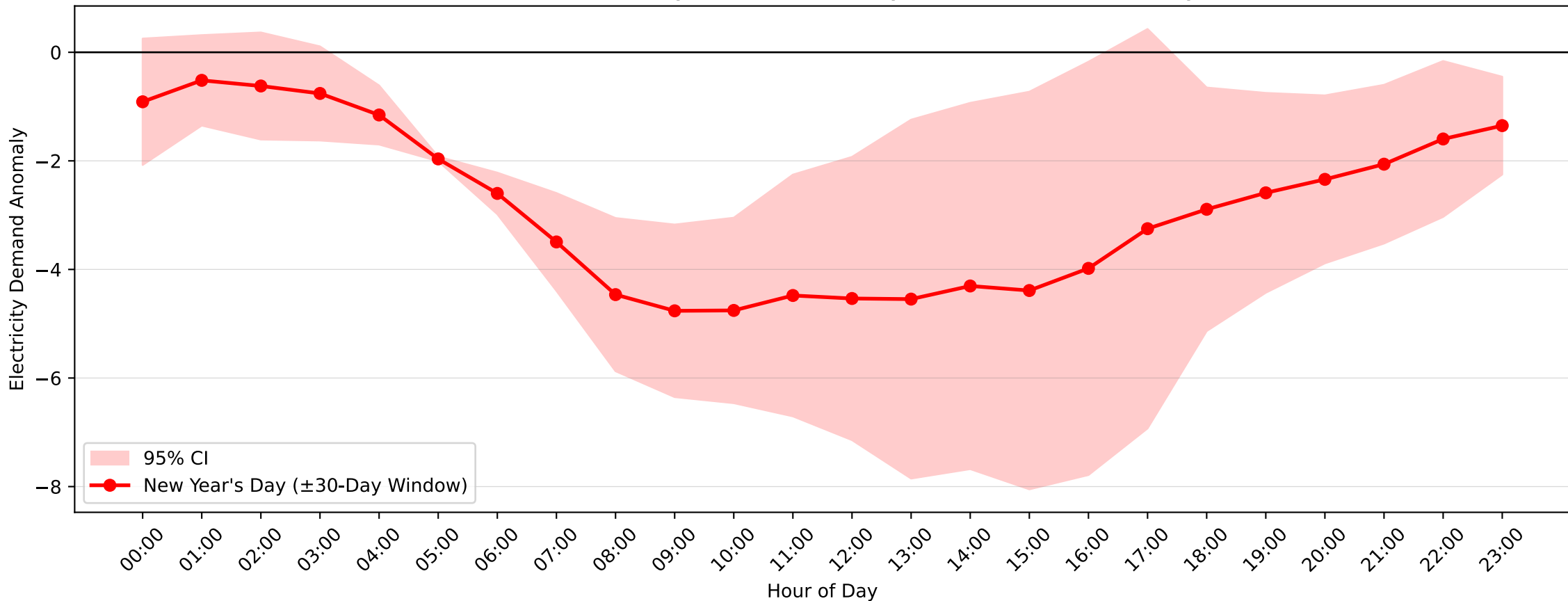
Lidcombe Demand Anomaly: New Year's Day (2007-2008, \pm 30 -Day Window)
