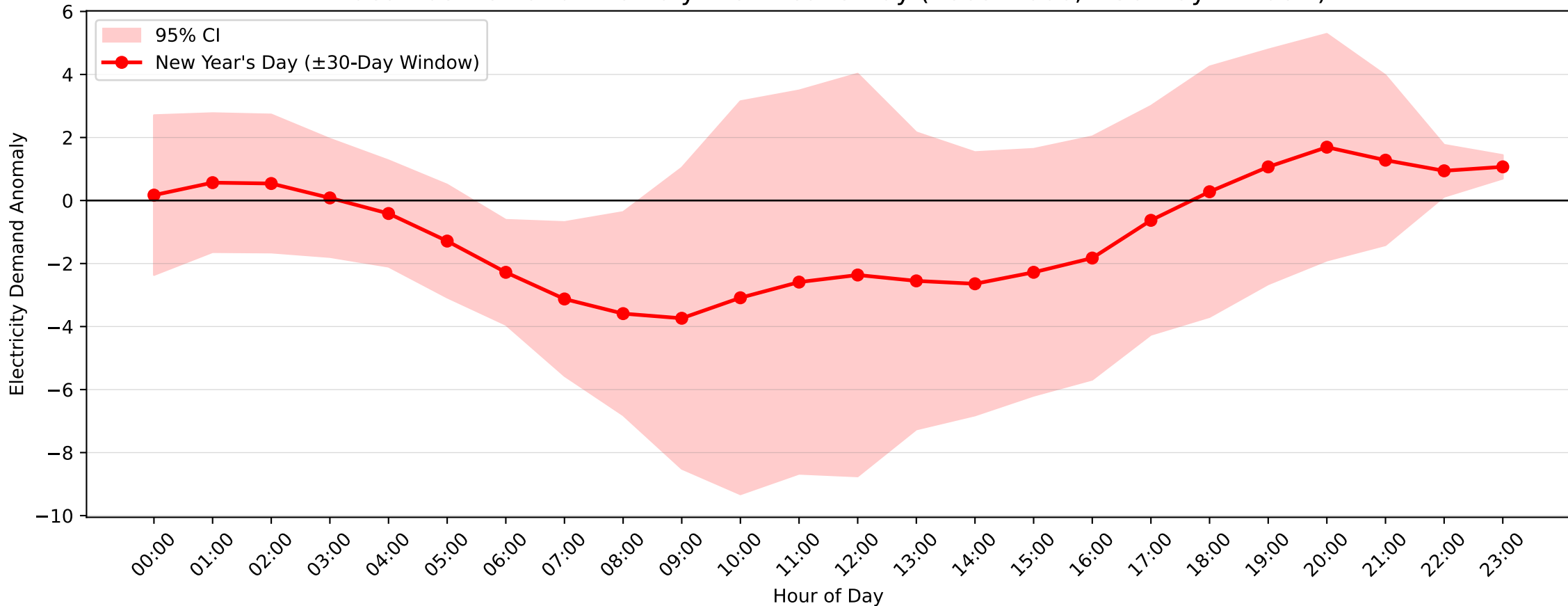
Lidcombe Demand Anomaly: New Year's Day (2005–2006, \pm 30 -Day Window)
