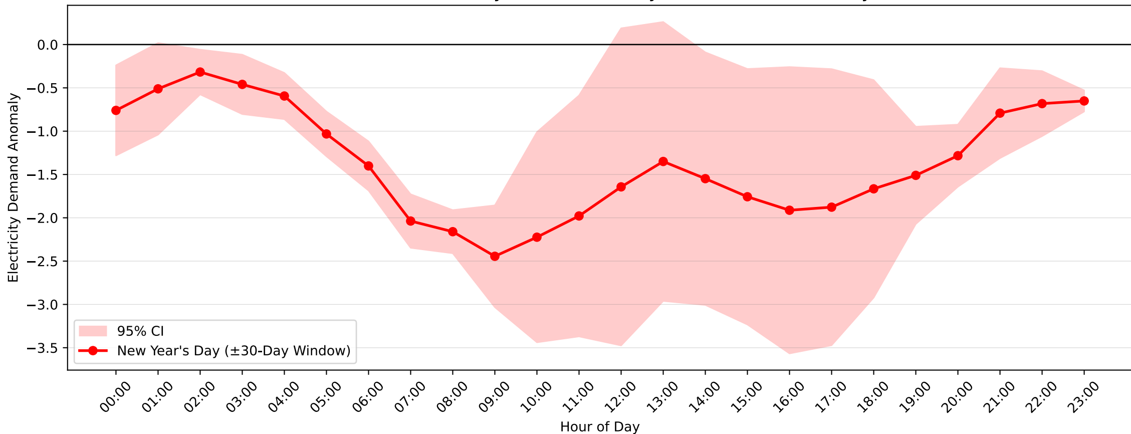
Lidcombe Demand Anomaly: New Year's Day (2013–2014, \pm 30 -Day Window)
