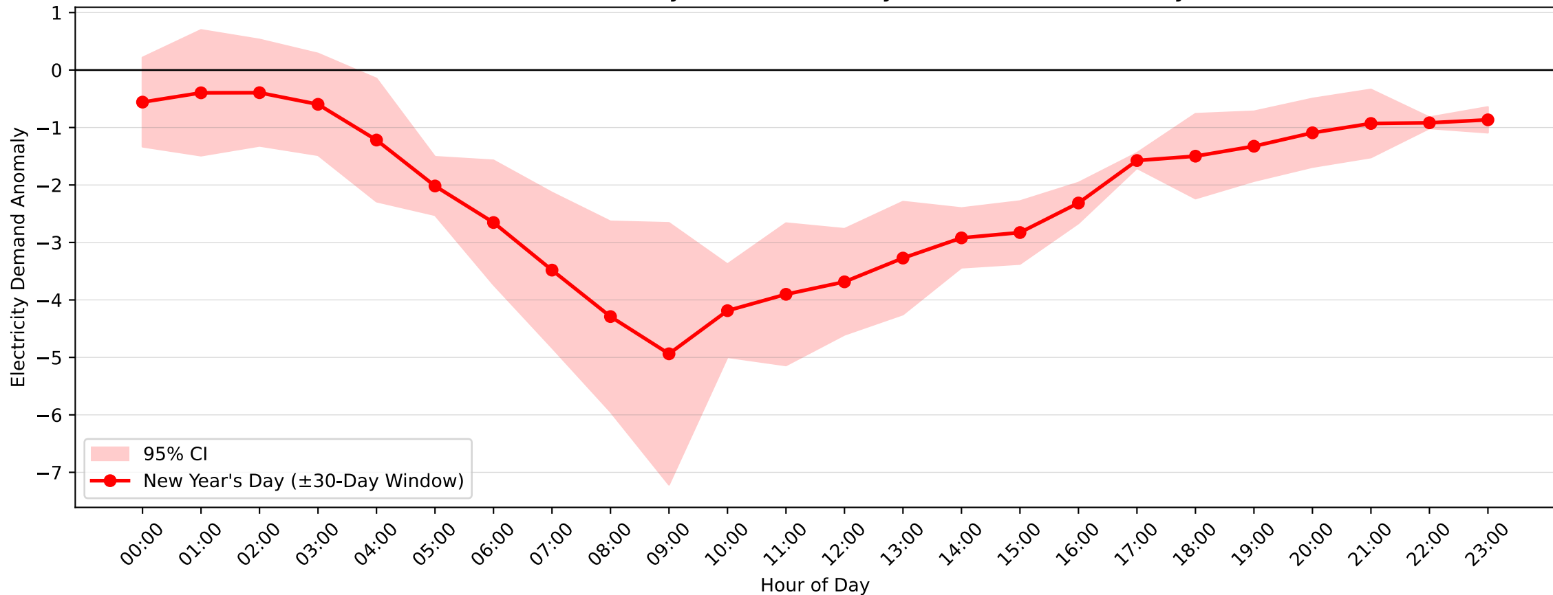
Lidcombe Demand Anomaly: New Year's Day (2008-2009, \pm 30 -Day Window)
