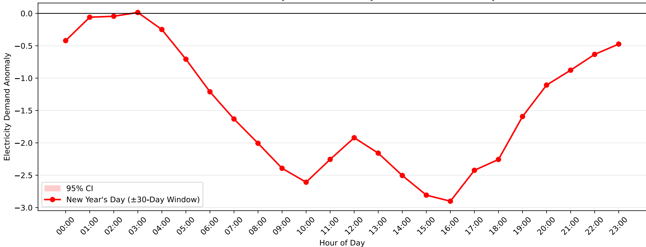
Lidcombe Demand Anomaly: New Year's Day (2017-2018, \pm 30 -Day Window)
