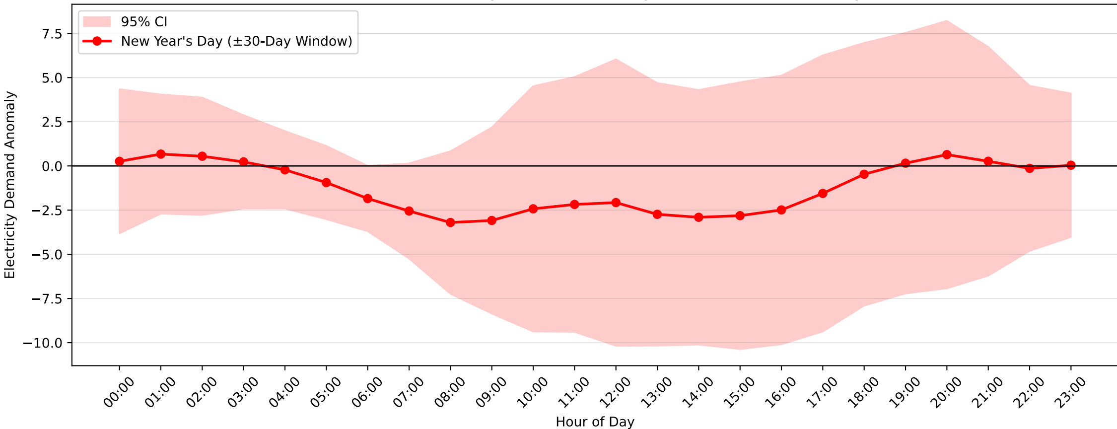
Lidcombe Demand Anomaly: New Year's Day (2006-2007, \pm 30 -Day Window)
